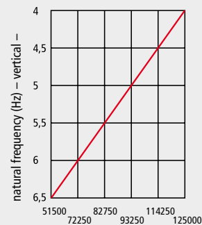
FAEBI® 580-HD load (N)
