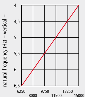
FAEBI® 200-HD load (N)
